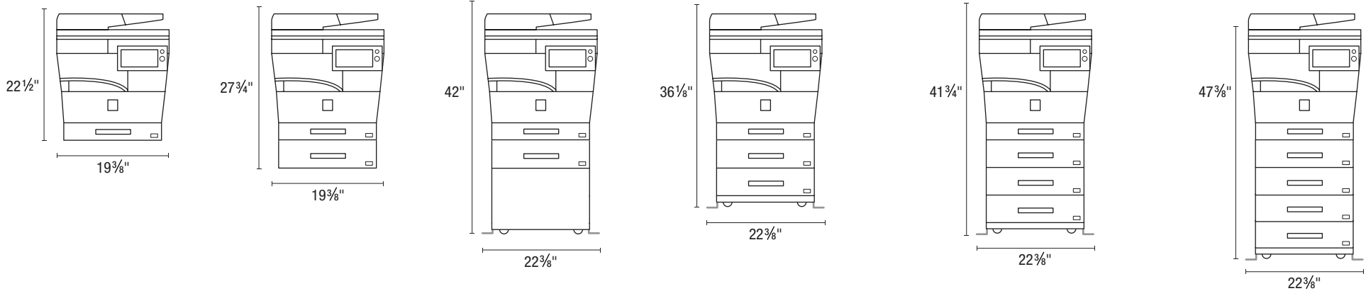
MX-C304W (standard drawer table top) 300-sheet maximum
