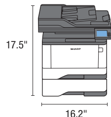
MX-B427W + MX-CS26 (1 additional drawer, table top) 900-sheet maximum
